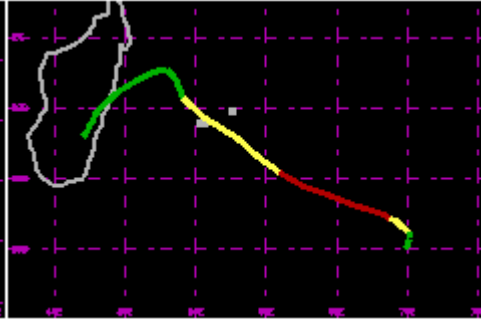
TC 22S Mar 1981 80kt
