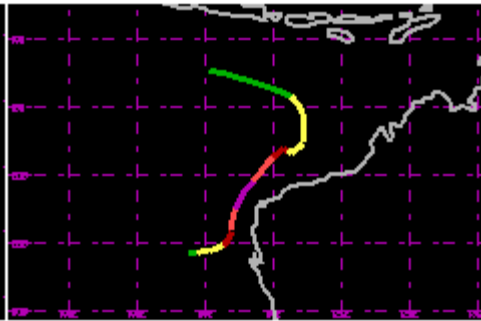
TC 10S Jan 1981 100kt
