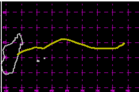
TC 03S Nov 1980 75kt
