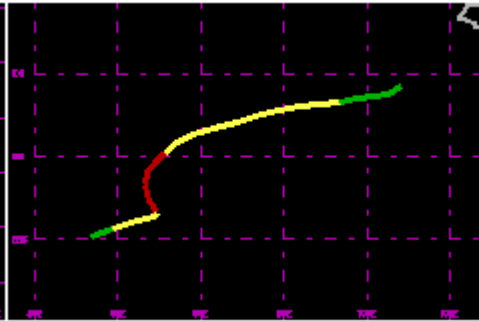
TC 28S Apr 1986 75kt
