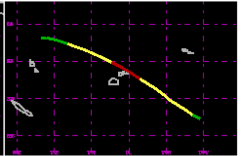
TC 29P Apr 1986 75kt
