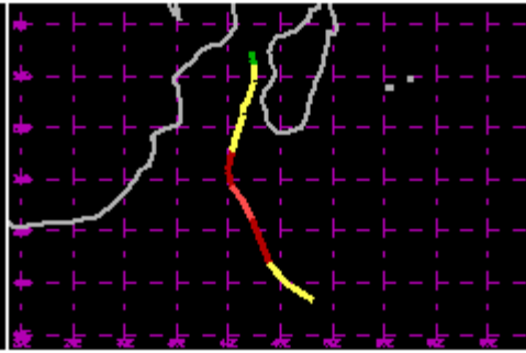
TC 19S Feb 1986 85kt
