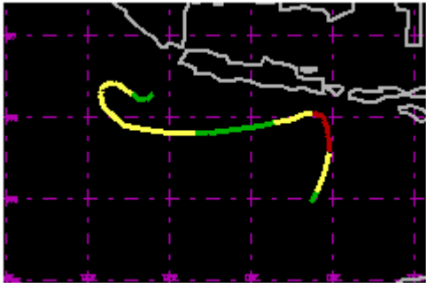
TC 02S Nov/Dec 1985 75kt
