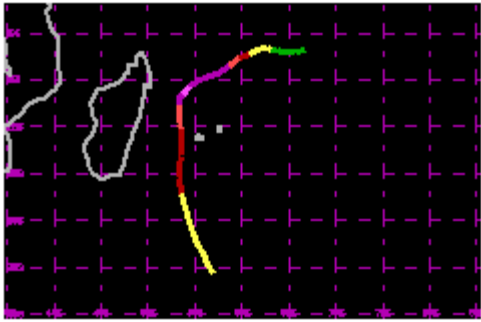
TC 13S Feb 1986 115kt
