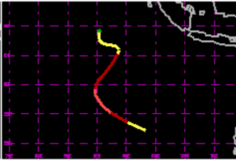
TC 32S Apr 1986 95kt
