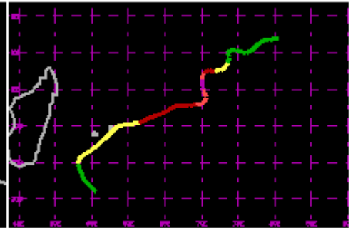
TC 21S Mar/Apr 1989 105kt
