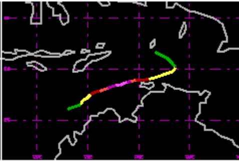
TC 28S Apr 1992 120kt
