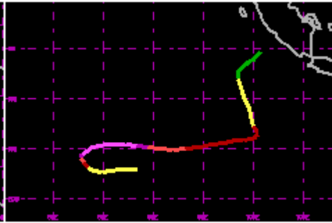
TC 29S Apr 1992 120kt
