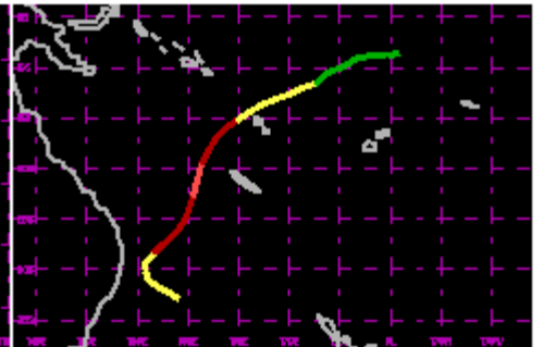
TC 17P Feb 1992 85kt
