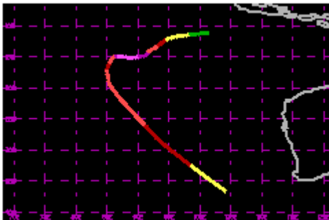
TC 20S Feb/Mar 1992 120kt
