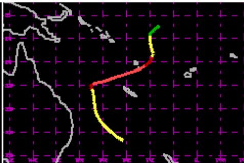
TC 11P Jan 1992 95kt
