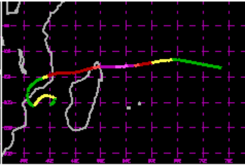
TC 23S Mar 1994 120kt
