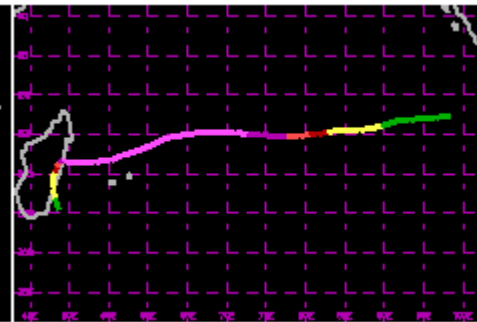
TC 20S Mar 1994 130kt
