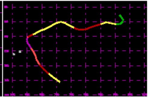
TC 26S Mar/Apr 1994 105kt
