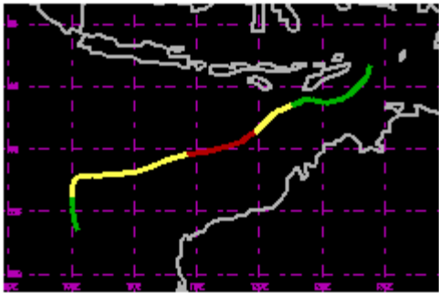
TC 28S Apr 1994 70kt
