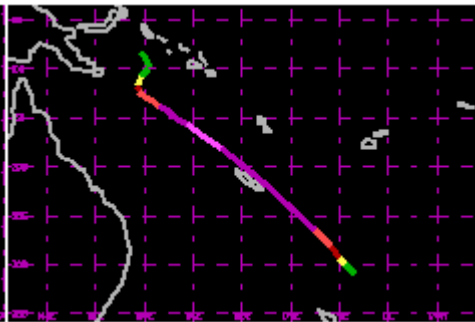
TC 18P Feb 1994 115kt
