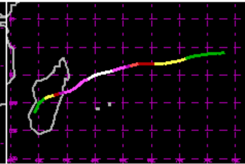
TC 13S Jan/Feb 1994 145kt
