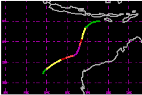
TC 22S Mar 1994 110kt
