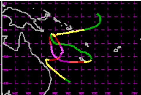
TC 05P Dec/Jan 1994 125kt
