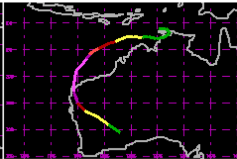
TC 30S Mar 1999 125kt
