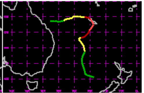
TC 22P Feb 1999 95kt
