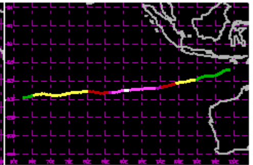
TC 31S Mar/Apr 1999 140kt
