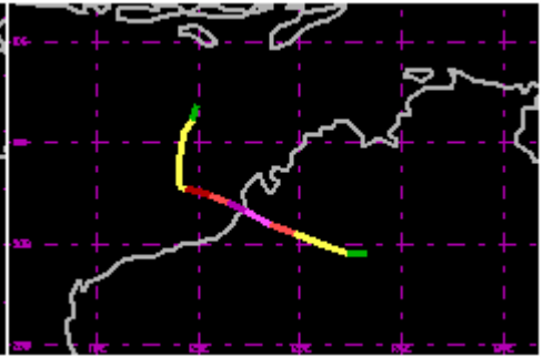
TC 27S Apr 2000 125kt
