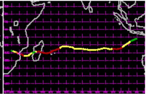
TC 11S Feb 2000 115kt
