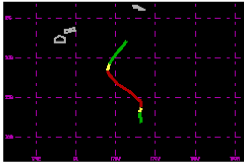
TC 19P Mar 2000 80kt
