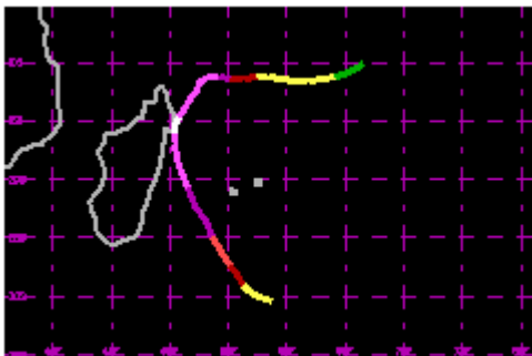
TC 18S Mar 2002 140kt
