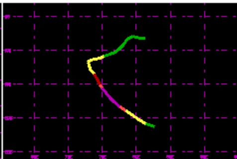
TC 20S Mar 2002 110kt
