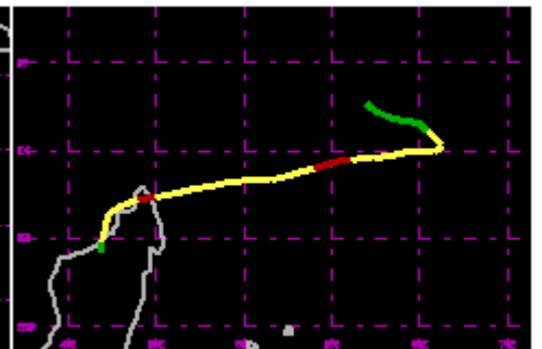
TC 23S May 2002 65kt
