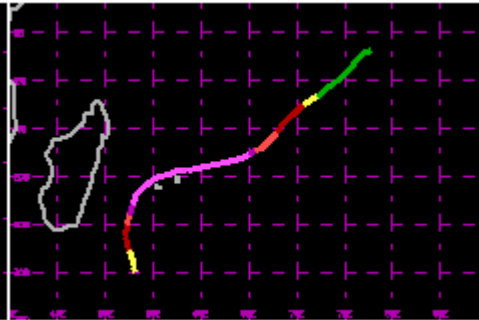
TC 10S Jan 2002 130kt
