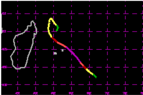
TC 16S Feb 2003 105kt
