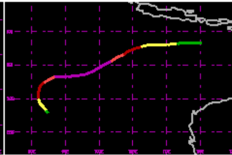
TC 14S Feb 2003 110kt
