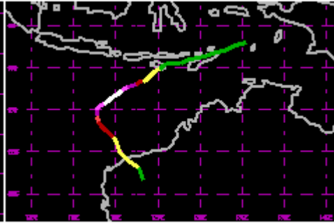
TC 26S Apr 2003 140kt
