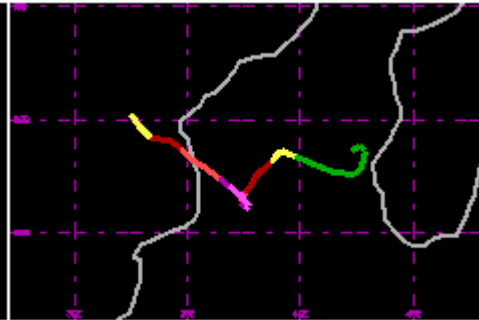
TC 19S Feb/Mar 2003 115kt
