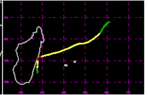
TC 28S May 2003 75kt
