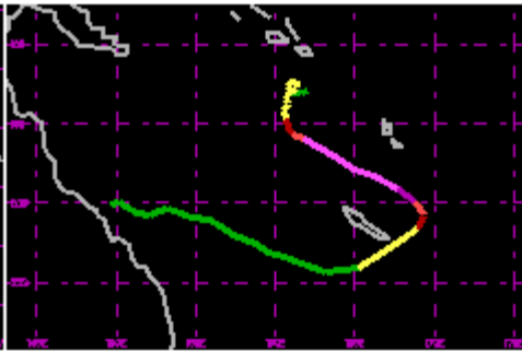
TC 12P Jan/Feb 2003 125kt
