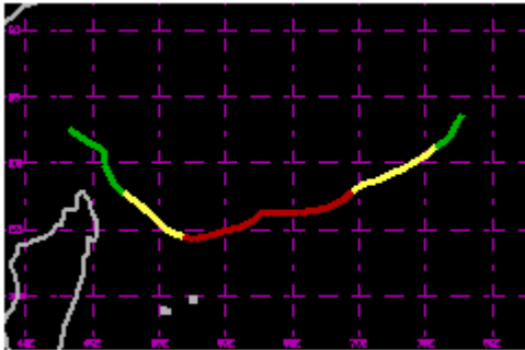
TC 03S Nov 2002 75kt
