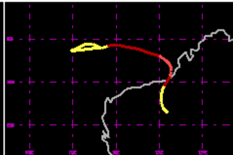
TC 16S Jan/Feb 85kt
