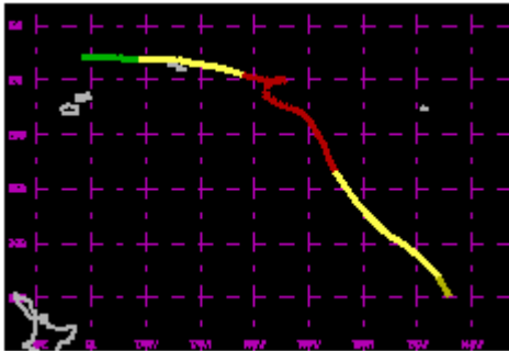
TC 20P Feb 1978 75kt
