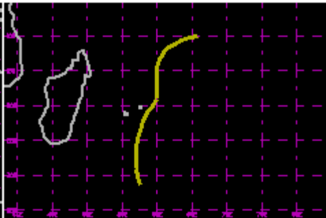
TC 13S Jan 1978
