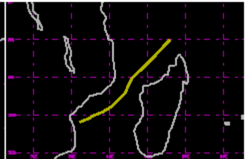
TC 18S Feb 1978 75kt
