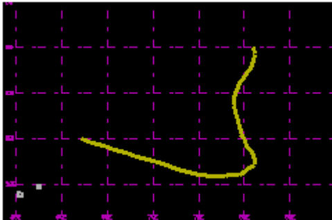
TC 02S Nov 1977
