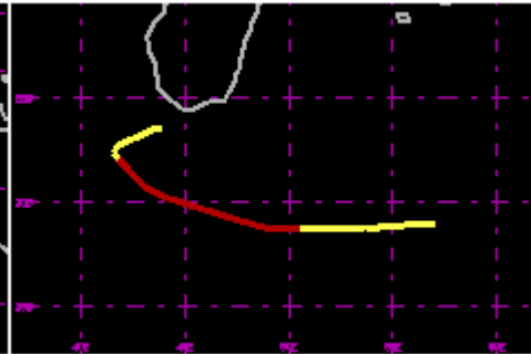
TC 24S Apr 1987 75kt
