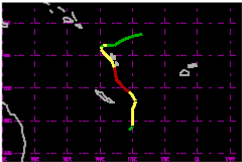
TC 19P Apr 2001 70kt
