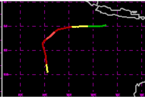
TC 17S Apr 2001 90kt
