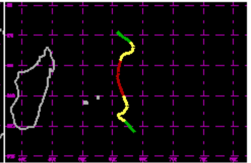
TC 18S Apr 2001 75kt
