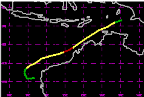
TC 20S Apr 2001 65kt
